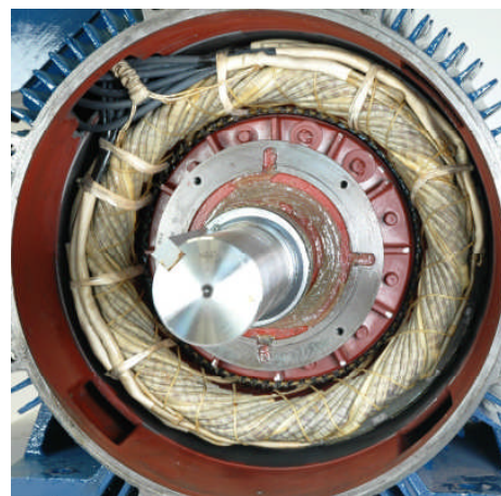
VPI and Fully Rapped End Turns
